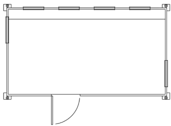
PK161 Ticket office 5.08 x 2.90m
