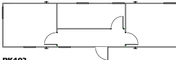
PK402 3 office unit 12.24 x 3.27m
