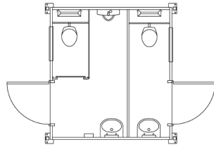
PL 101 (type C) Male/Female toilet unit 3.08 x 2.90m
