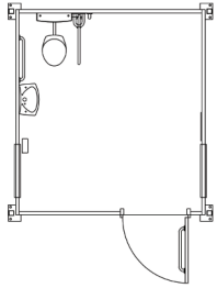
PL 101 (type A) Disabled persons toilet unit Mains: 3.08 x 2.90m
