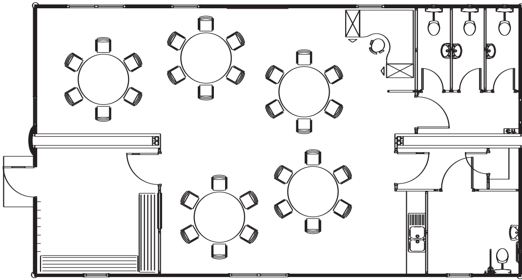
Primary classroom with entrance lobby, toilet facilities and wet play area –floor area 110.56m 2 2 TN154's
