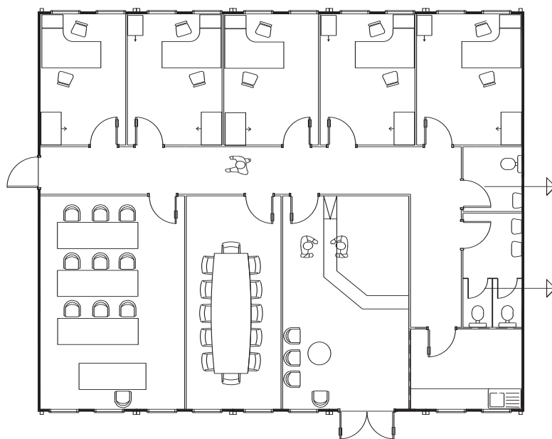
UK093 Ultima office complex - floor area 155.80m 2
